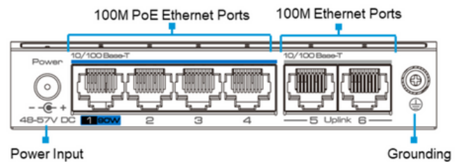
Top Panel
