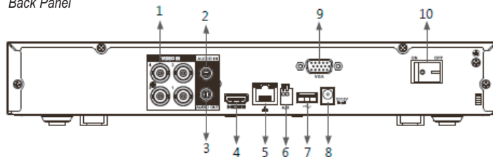
Back Panel
