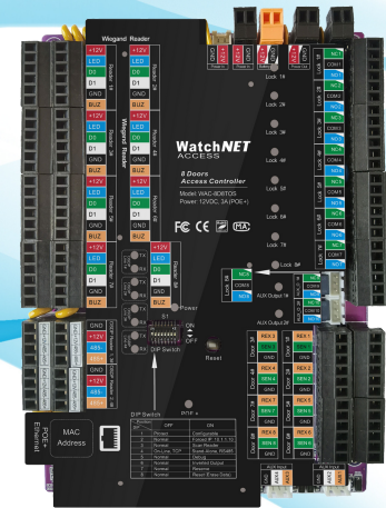
WAC-8D8TOS-PCB
