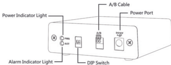
Front Panel
