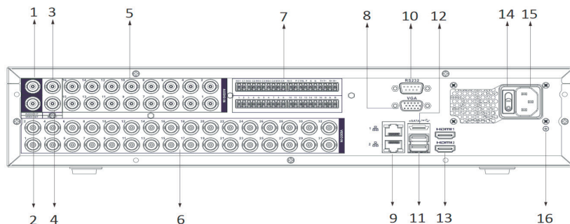
Back Panel
